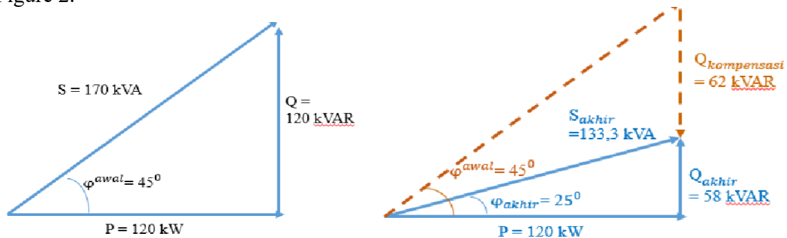
Figure 2. Reactive Power Compensation Analysis (a) Power triangle condition when power factor (Pf) = 0.7 lagging (b) Power triangle condition when power factor (Pf) = 0.9 lagging.
