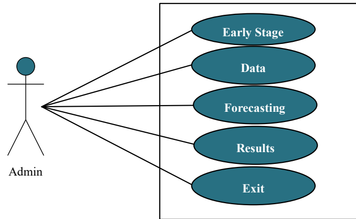
Figure 1. Use Case
