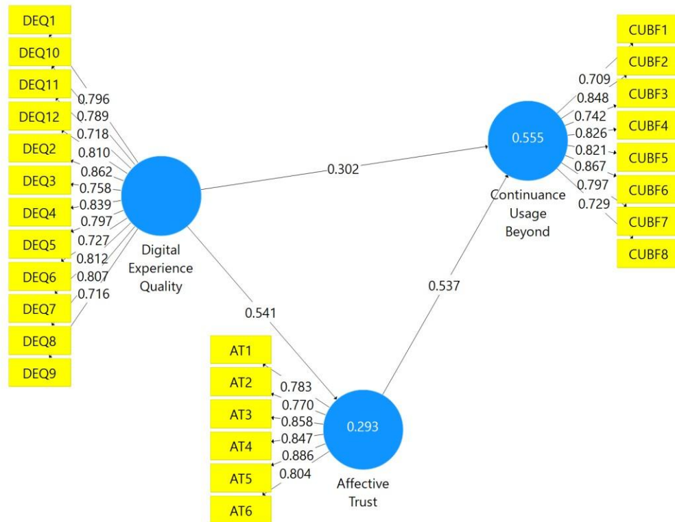
Figure 2. PLS-SEM Algorithm
