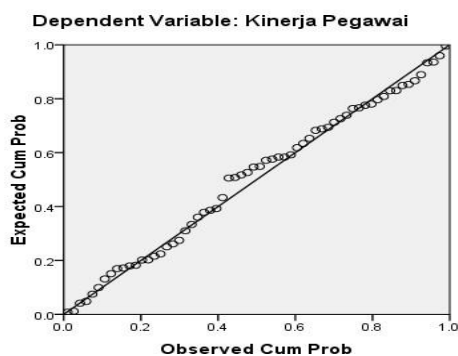
Figure 3. PP Normality Test Plot
