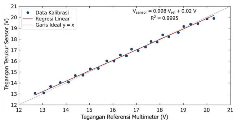
Figure 3. Chart DC voltage sensor calibration against multimeter
