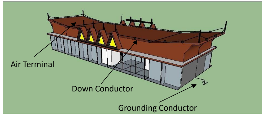
Figure 3. Lightning Protection Installation on the Sugimanuru Airport Terminal Building
