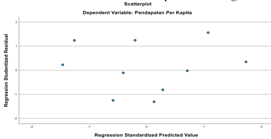
Figure 1. Heteroscedasticity Test Graph
