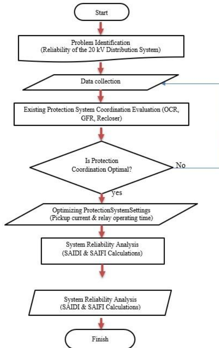
Figure 1. Research Flowchart
