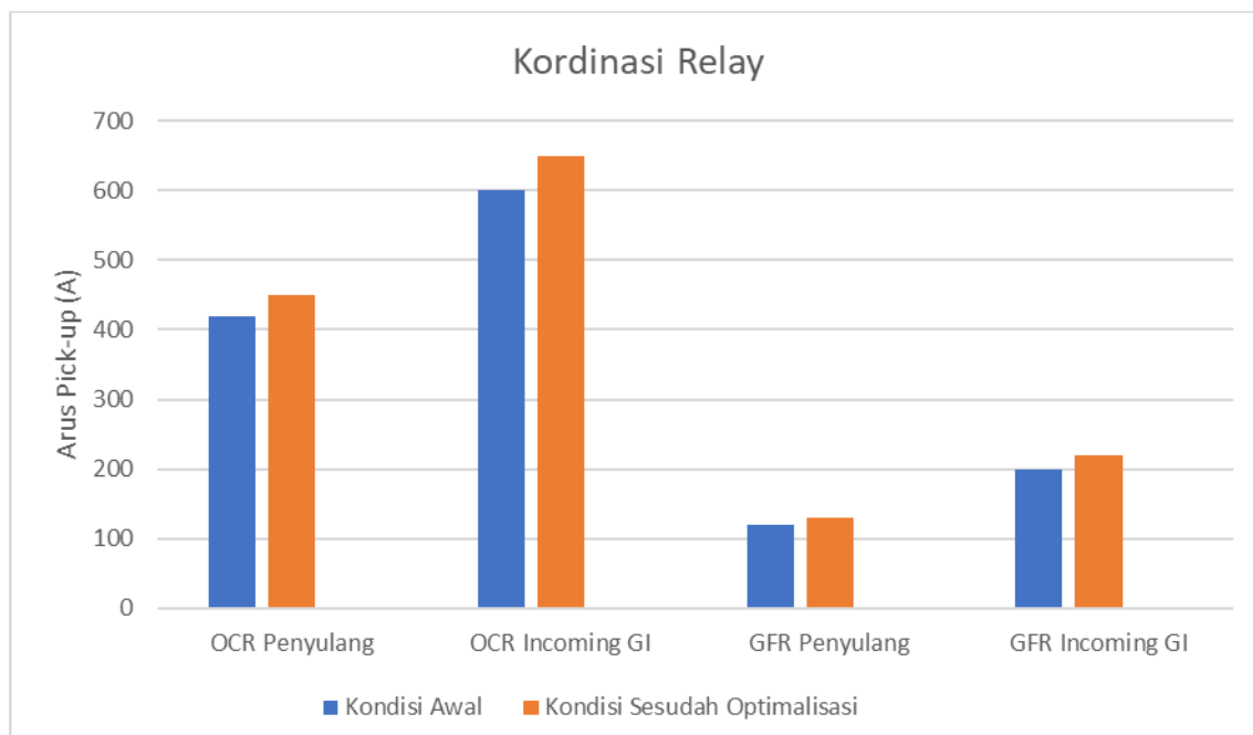
Figure 2. Relay Coordination Graph Before and After Optimization
