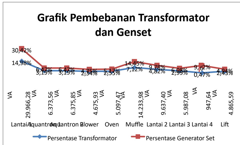
Figure 6. Load Graph of Transformers and Generators
