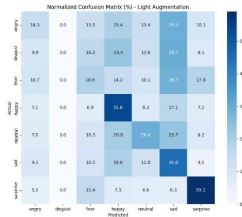
Figure 5. Normalized Confusion Matrix (%) for Light Augmentation Model
