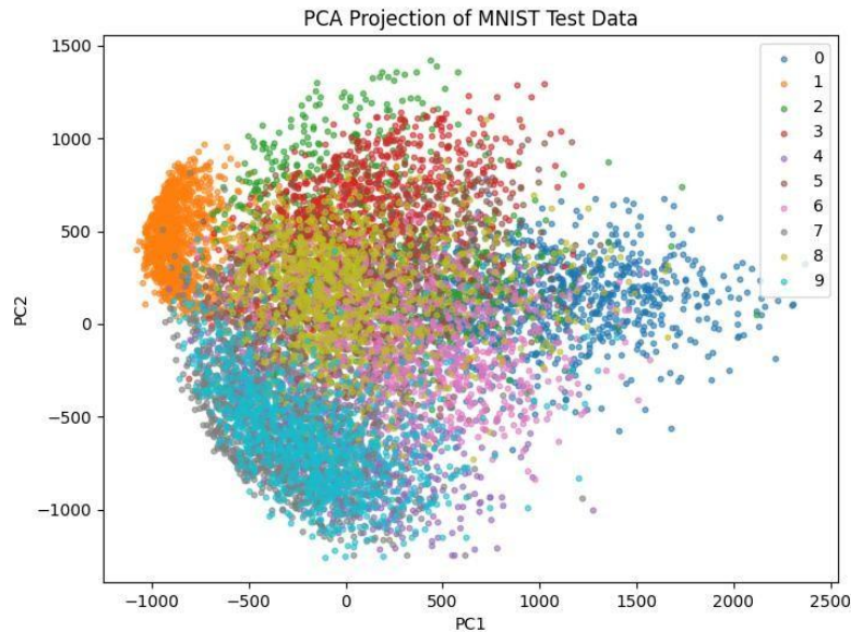
Figure 3. PCA Plot
