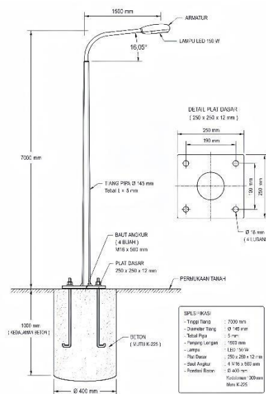
Figure 4. Public Street Lighting Laying Simulation 7)
