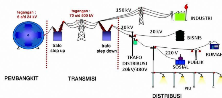
Figure 1. Energy source flow in the Public Street Lighting system
