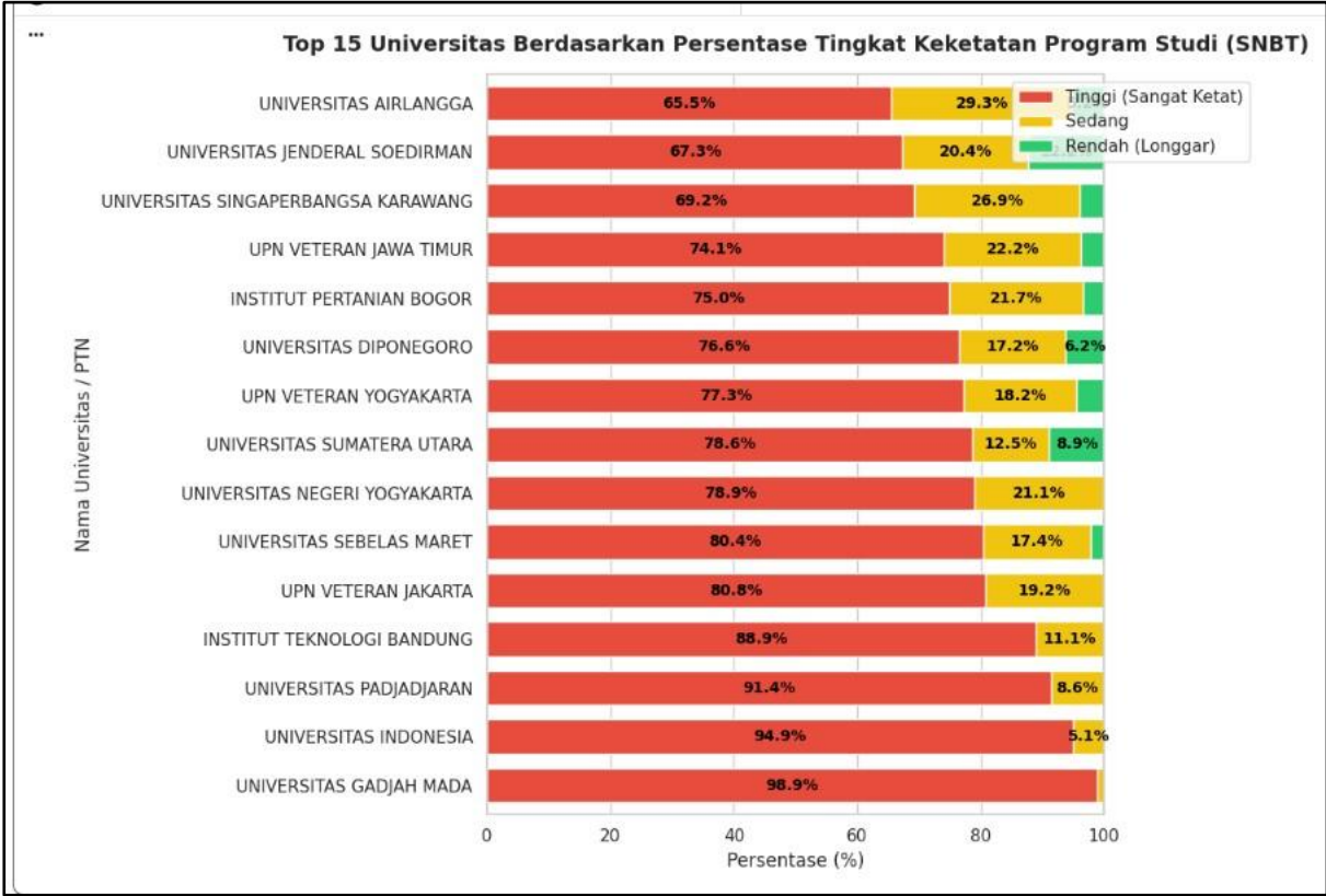
Figure 4. Horizontal Bar Visualization of the Randome Forest Model
