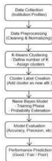
Figure 1. Naive Bayes And K-Means Clustering Process Diagram Process Diagram
