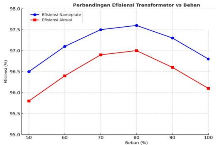
Figure 4. Comparison of Transformer Efficiency
