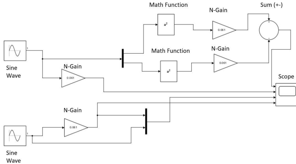
Figure 5. Simulink Modeling
