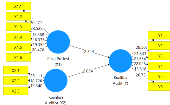
Figure 6. Bootstrapping Testing Based on Outer Loading
