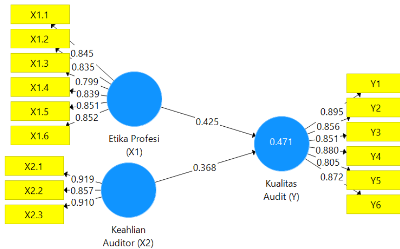
Figure 2. Validity Testing by Loading Factor
