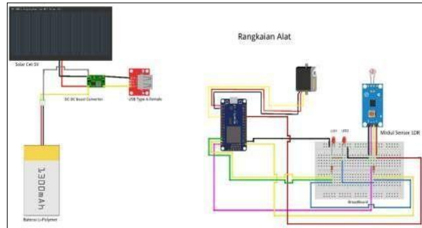
Figure 3. Circuit Schematic
